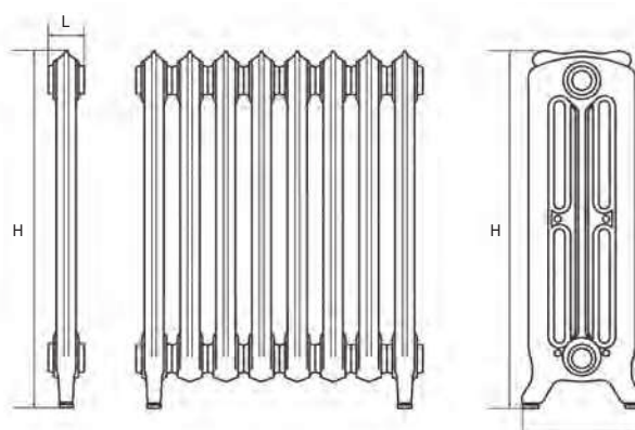
Anschlüsse/Raccordement: 4x 1/2"
