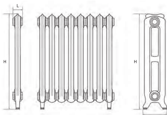
Anschlüsse/Raccordement: 4x 1/2"
