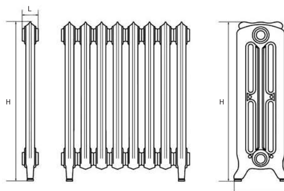
Anschlüsse/Raccordement: 4x 1/2"
