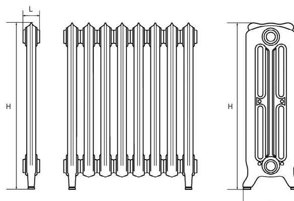
Anschlüsse/Raccordement: 4x 1/2"
